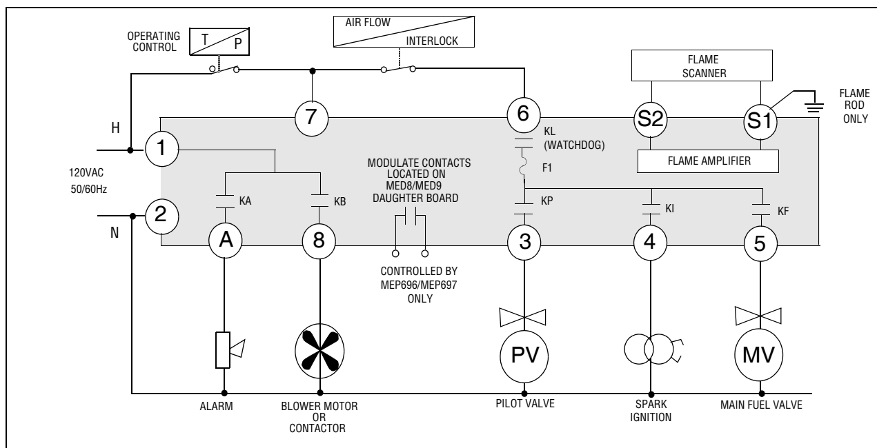
FIGURE 12. WIRING ARRANGEMENT FOR PILOT IGNITED BURNERS USING MEP300, MEP400 AND MEP600 SERIES PROGRAMMERS.
